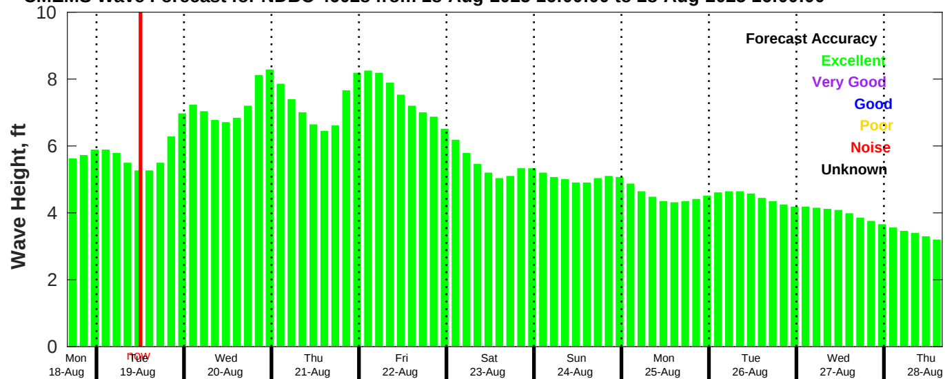
CMEMS Wave Forecast for NDBC 46028 from 18-Aug-2025 16:00:00 to 28-Aug-2025 16:00:00
