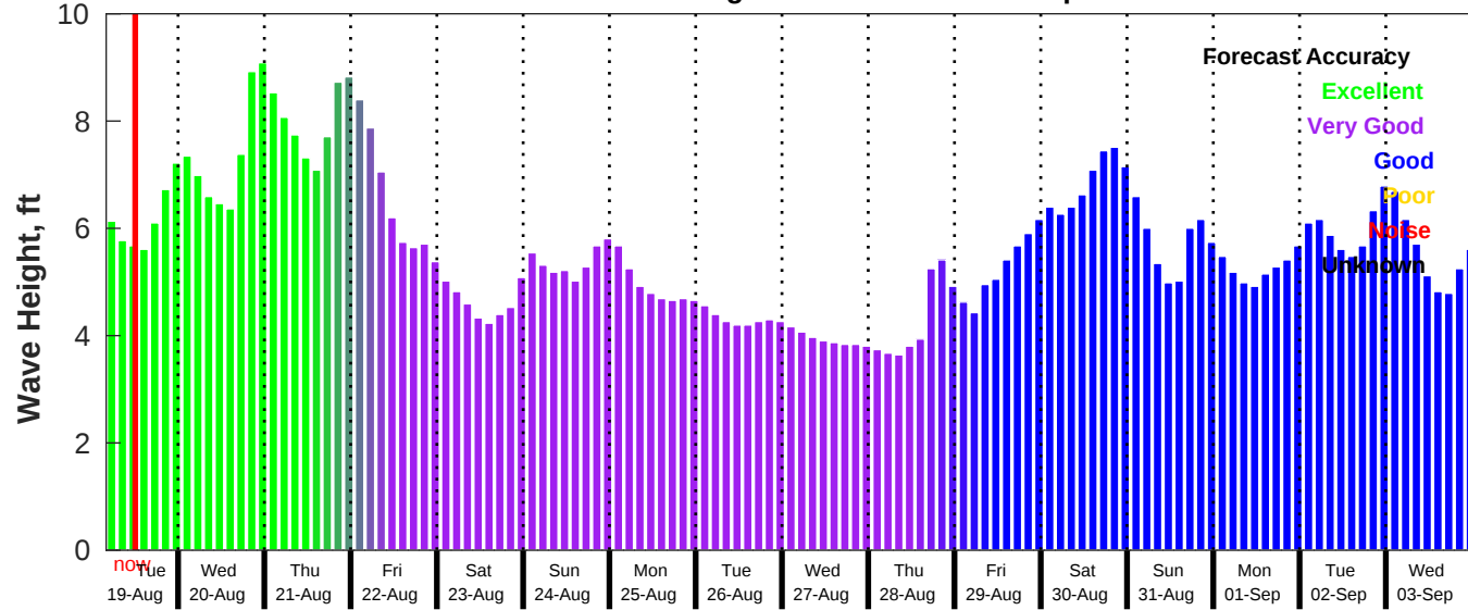
GFS Wave Forecast for NDBC 46028 from 19-Aug-2025 04:00:00 to 04-Sep-2025 04:00:00
