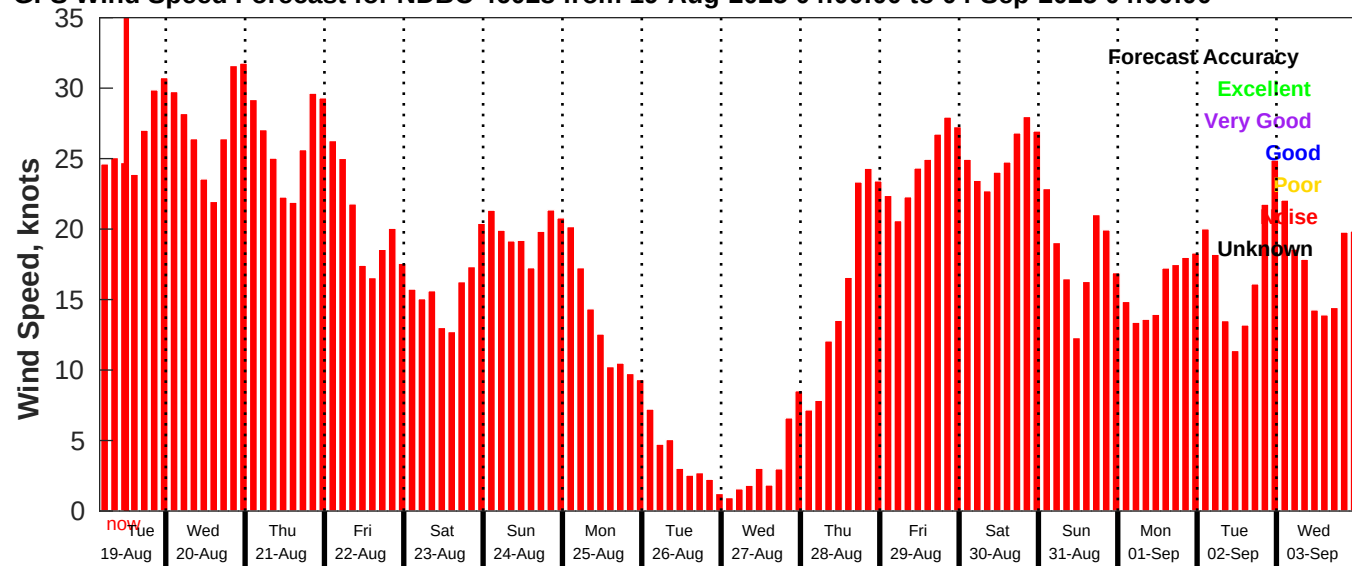
GFS Wind Speed Forecast for NDBC 46028 from 19-Aug-2025 04:00:00 to 04-Sep-2025 04:00:00
