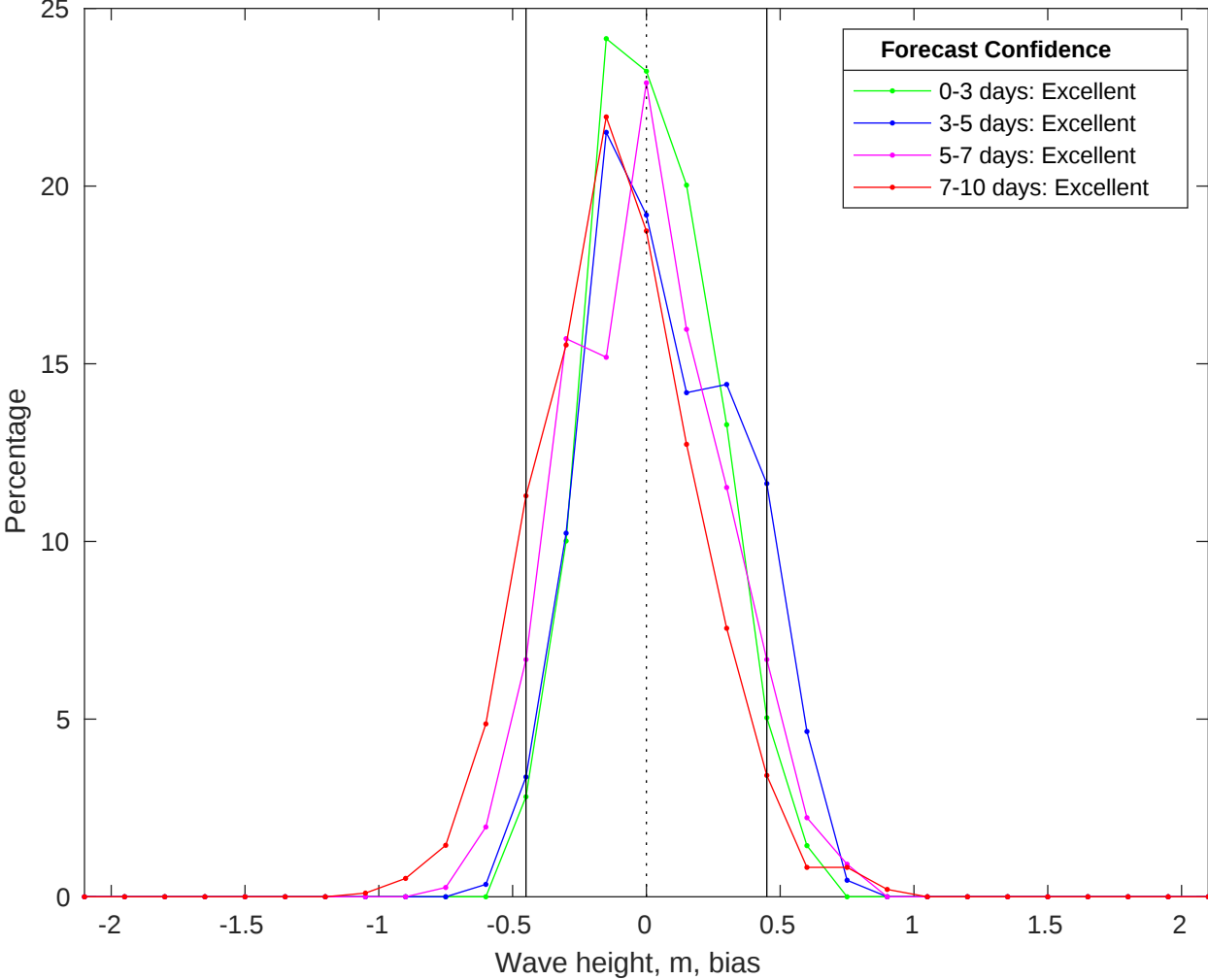
NDBC 46054 vs CMEMS Waves Bias Histogram: 19-Aug-2025
