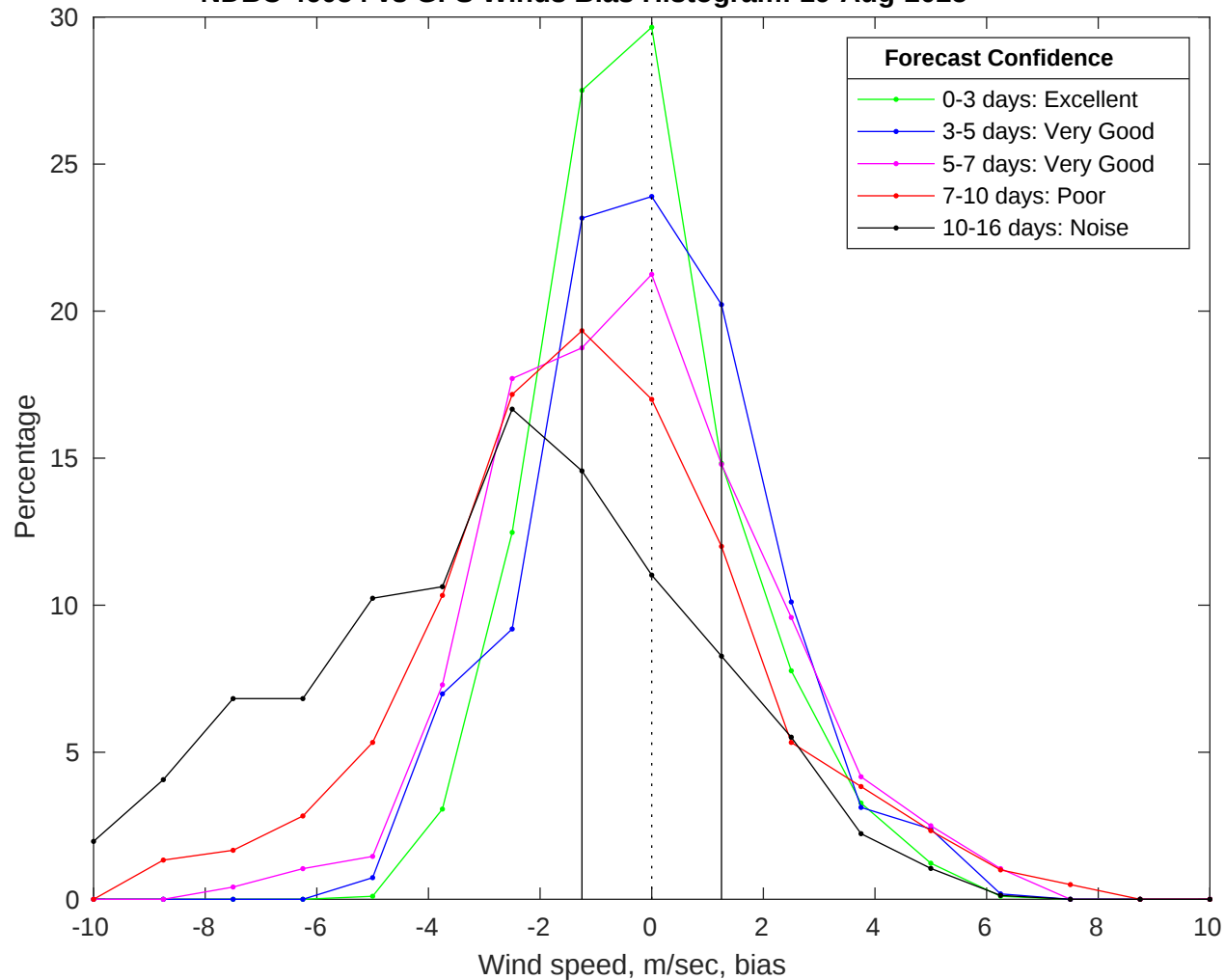
NDBC 46054 vs GFS Winds Bias Histogram: 19-Aug-2025
