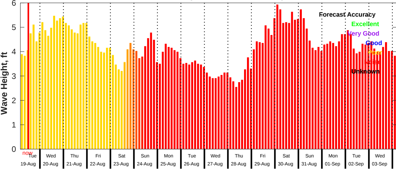
GFS Wave Forecast for NDBC 46054 from 19-Aug-2025 04:00:00 to 04-Sep-2025 04:00:00
