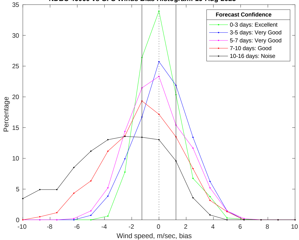
NDBC 46069 vs GFS Winds Bias Histogram: 19-Aug-2025
