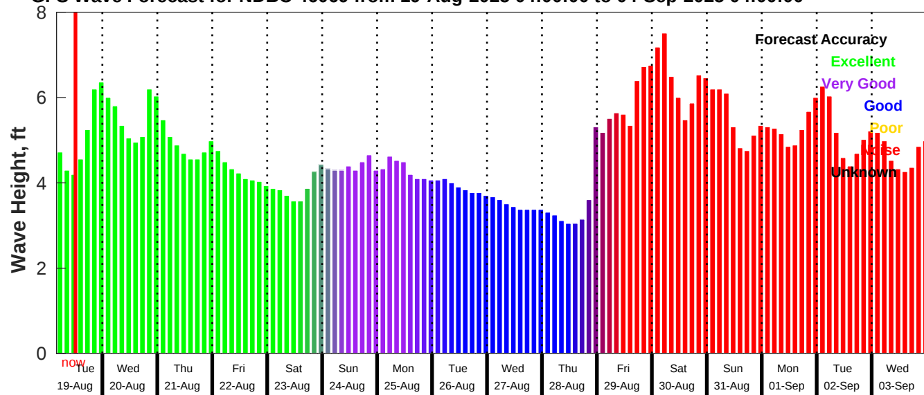
GFS Wave Forecast for NDBC 46069 from 19-Aug-2025 04:00:00 to 04-Sep-2025 04:00:00
