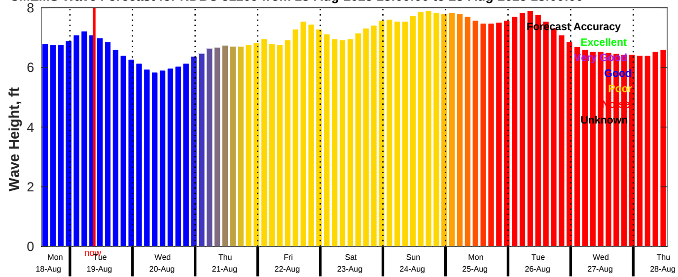
CMEMS Wave Forecast for NDBC 51209 from 18-Aug-2025 13:00:00 to 28-Aug-2025 13:00:00
