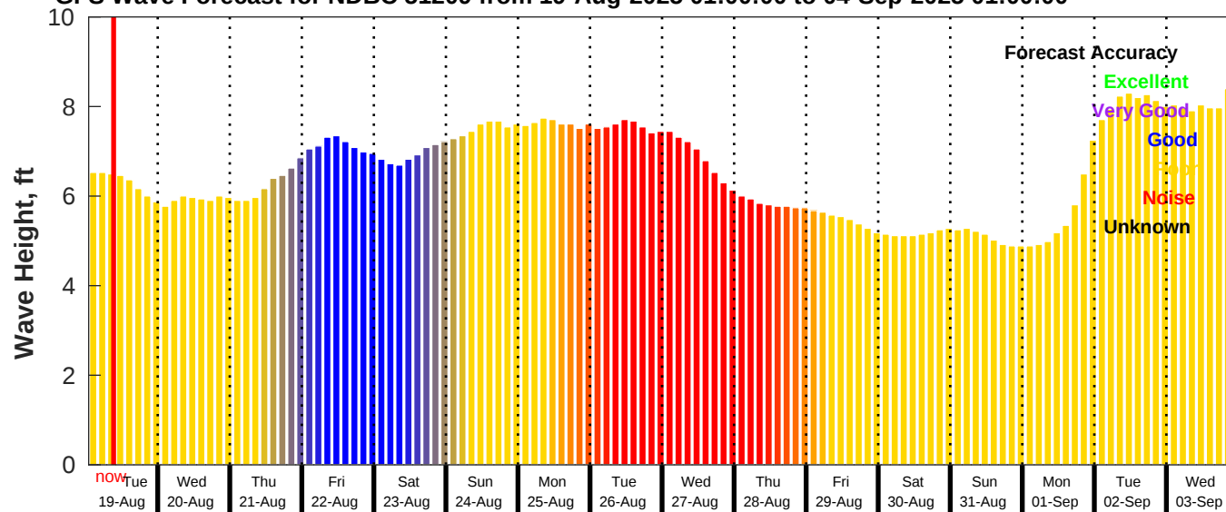
GFS Wave Forecast for NDBC 51209 from 19-Aug-2025 01:00:00 to 04-Sep-2025 01:00:00
