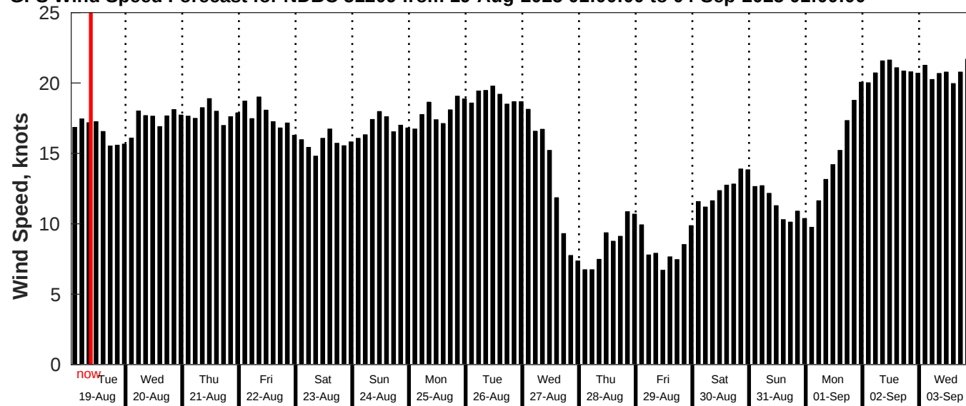
GFS Wind Speed Forecast for NDBC 51209 from 19-Aug-2025 01:00:00 to 04-Sep-2025 01:00:00
