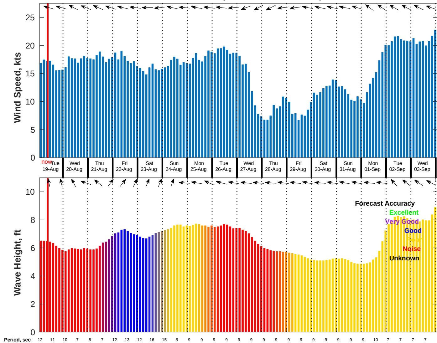
Wind & Wave Forecast for NDBC 51209 from 19-Aug-2025 01:00:00 to 04-Sep-2025 01:00:00
