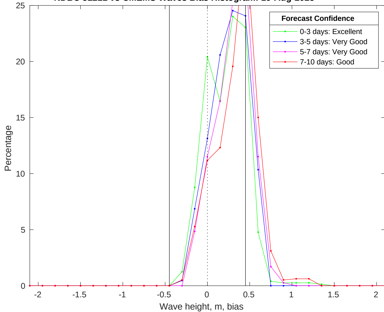
NDBC 51211 vs CMEMS Waves Bias Histogram: 19-Aug-2025
