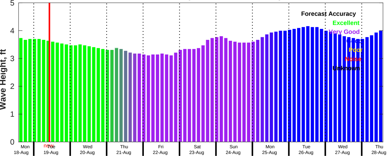
CMEMS Wave Forecast for NDBC 51211 from 18-Aug-2025 14:00:00 to 28-Aug-2025 14:00:00
