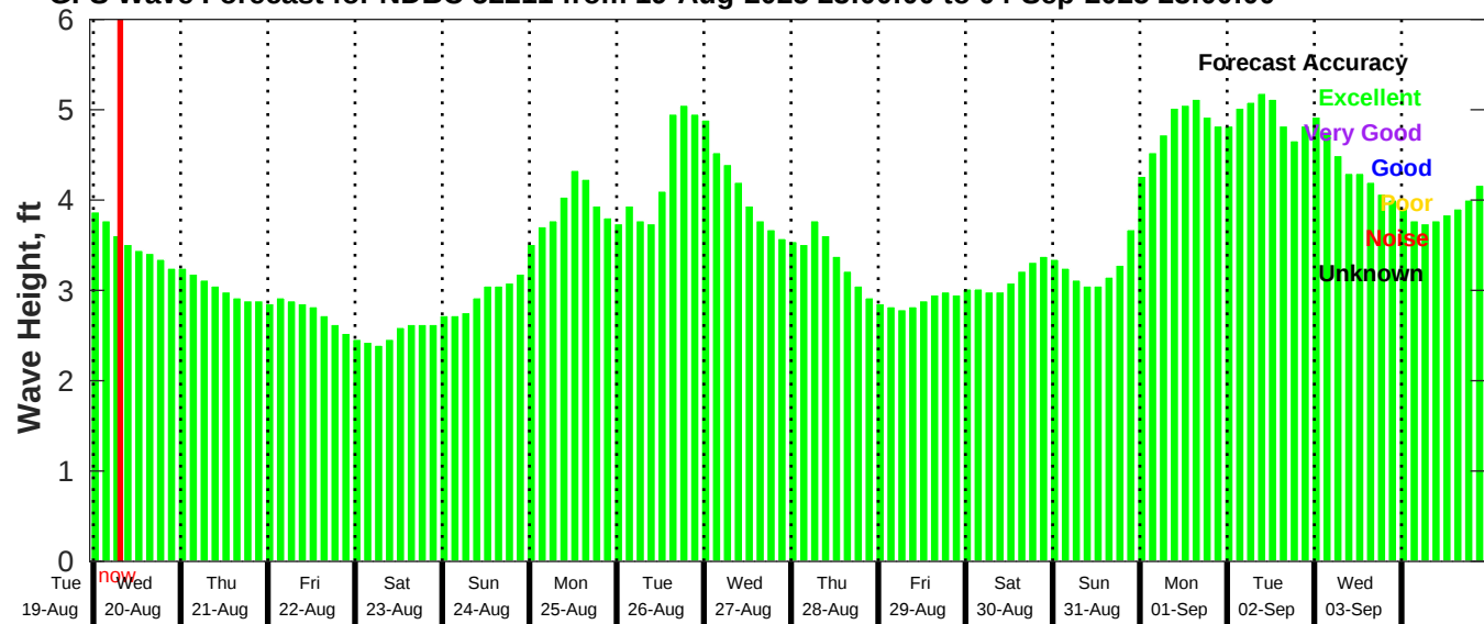
GFS Wave Forecast for NDBC 52211 from 19-Aug-2025 23:00:00 to 04-Sep-2025 23:00:00
