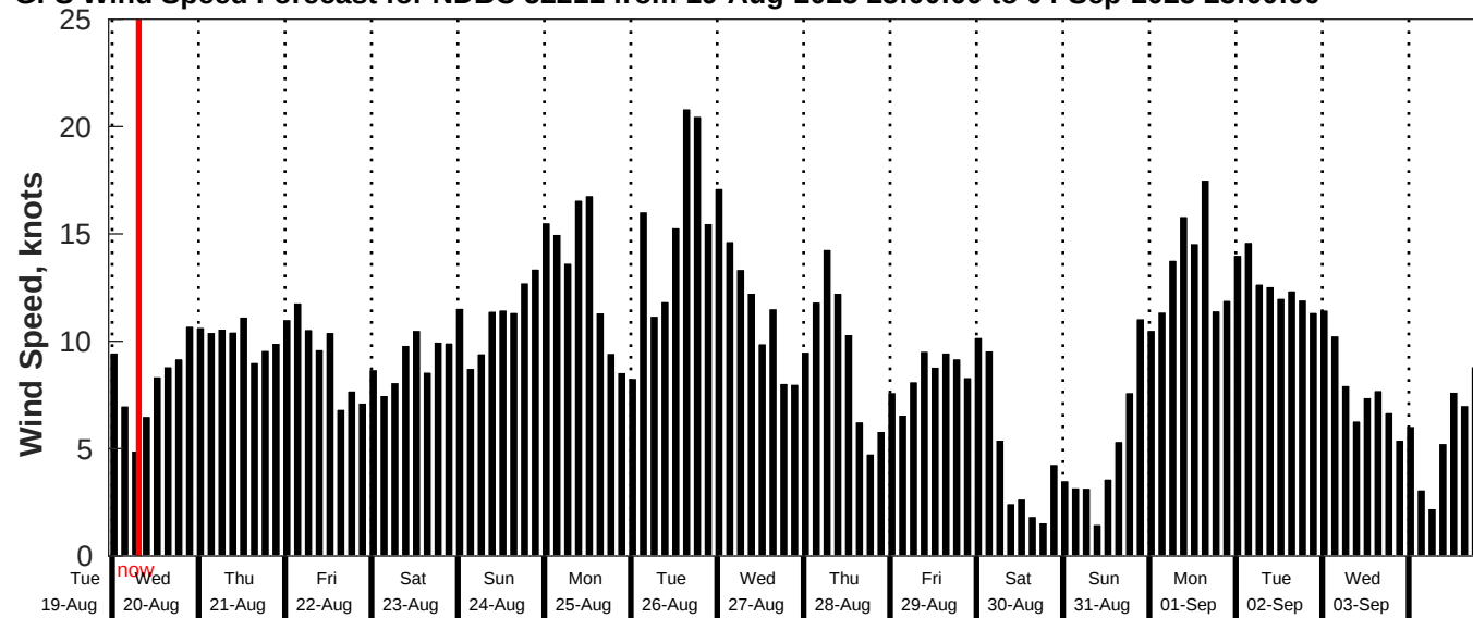
GFS Wind Speed Forecast for NDBC 52211 from 19-Aug-2025 23:00:00 to 04-Sep-2025 23:00:00
