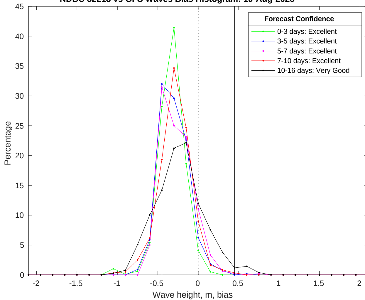
NDBC 52213 vs GFS Waves Bias Histogram: 19-Aug-2025
