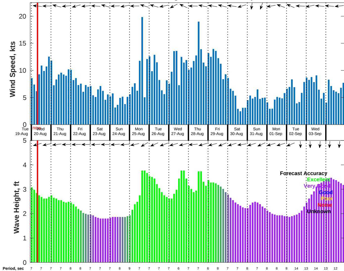
Wind & Wave Forecast for NDBC 52213 from 19-Aug-2025 23:00:00 to 04-Sep-2025 23:00:00
