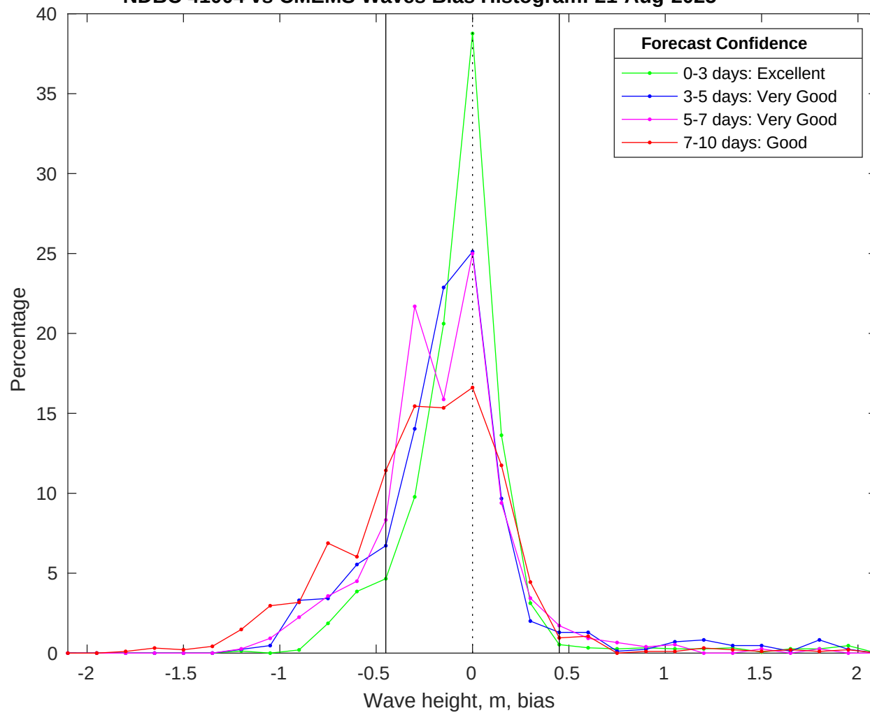
NDBC 41004 vs CMEMS Waves Bias Histogram: 21-Aug-2025
