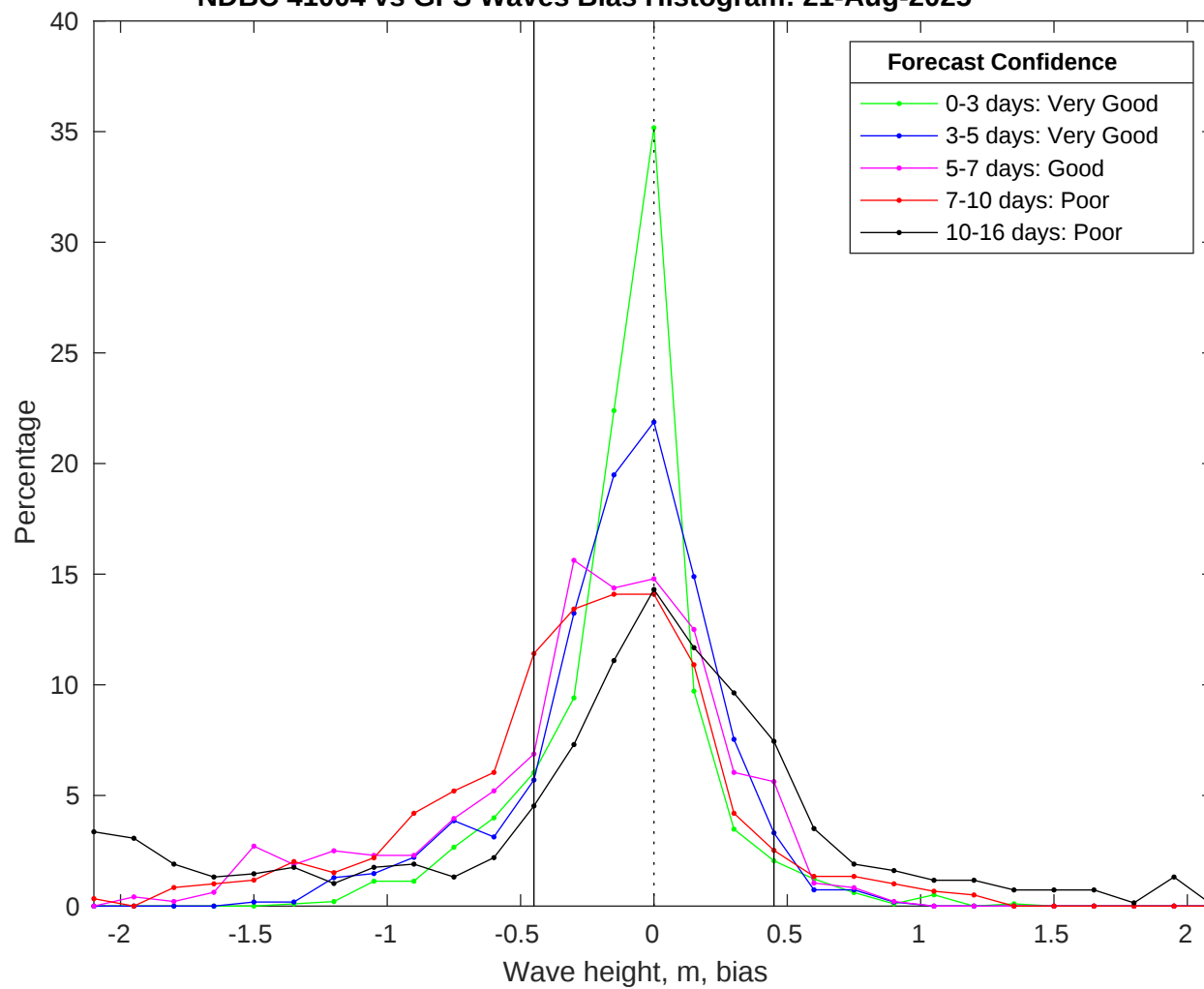
NDBC 41004 vs GFS Waves Bias Histogram: 21-Aug-2025
