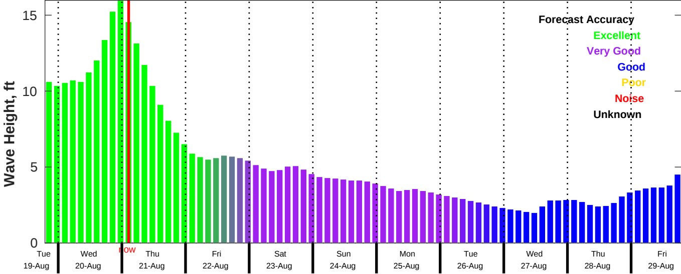
CMEMS Wave Forecast for NDBC 41004 from 19-Aug-2025 19:00:00 to 29-Aug-2025 19:00:00
