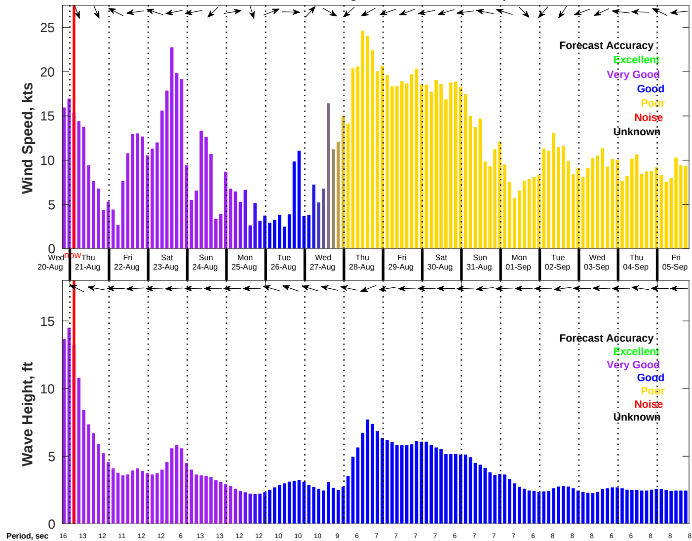
Wind & Wave Forecast for NDBC 41004 from 20-Aug-2025 19:00:00 to 05-Sep-2025 19:00:00
