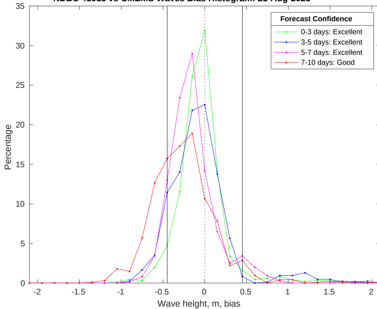
NDBC 41013 vs CMEMS Waves Bias Histogram: 21-Aug-2025
