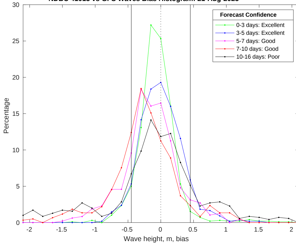
NDBC 41013 vs GFS Waves Bias Histogram: 21-Aug-2025
