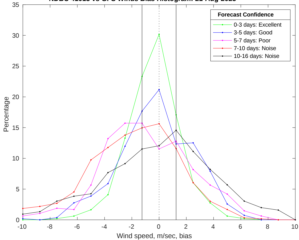
NDBC 41013 vs GFS Winds Bias Histogram: 21-Aug-2025
