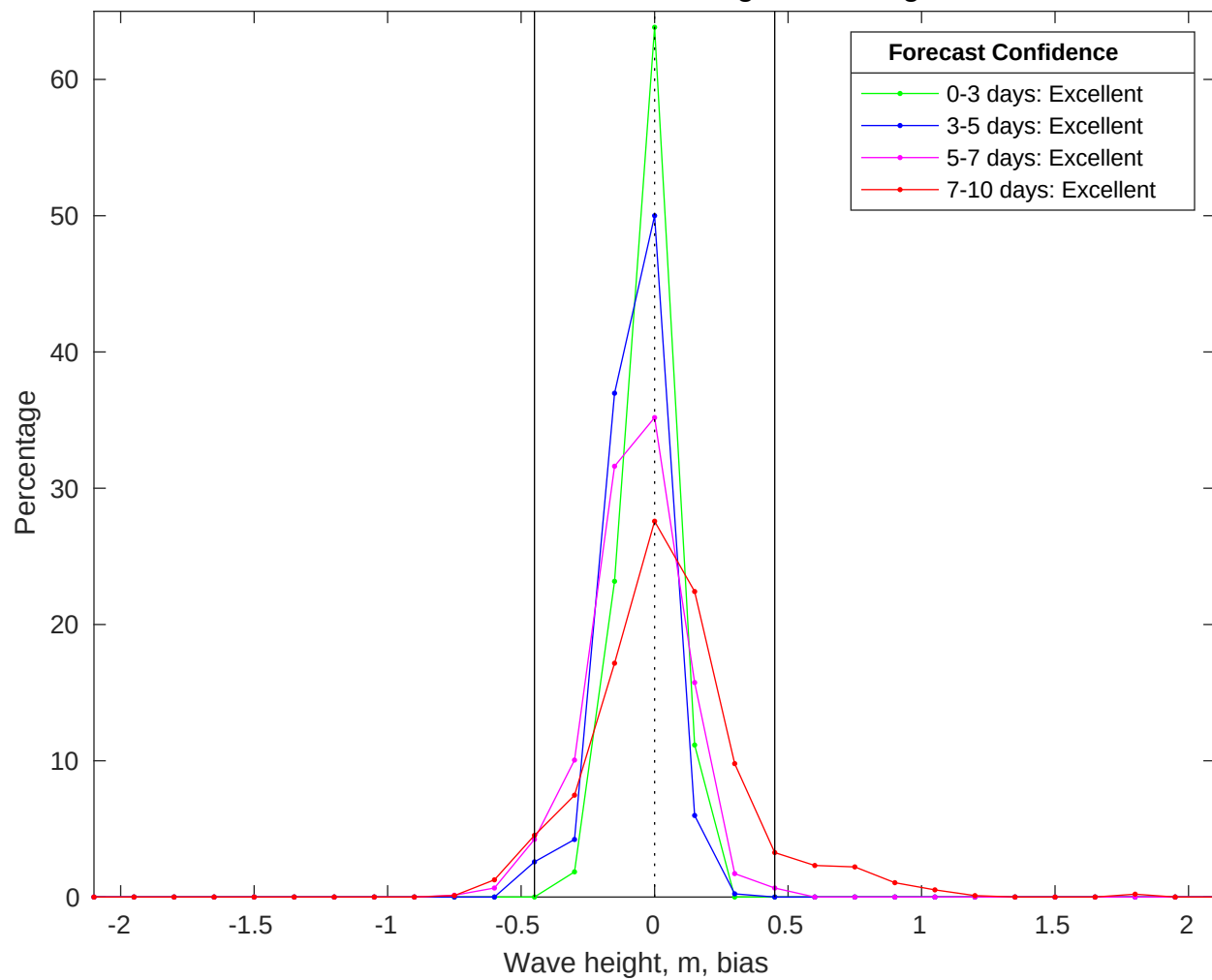
NDBC 41040 vs CMEMS Waves Bias Histogram: 21-Aug-2025
