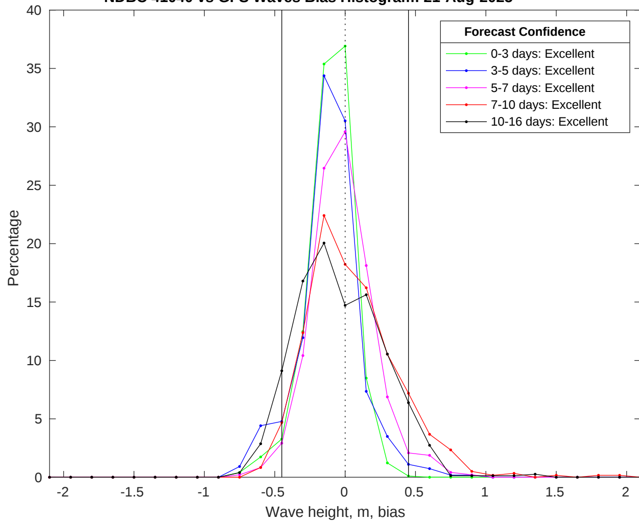
NDBC 41040 vs GFS Waves Bias Histogram: 21-Aug-2025
