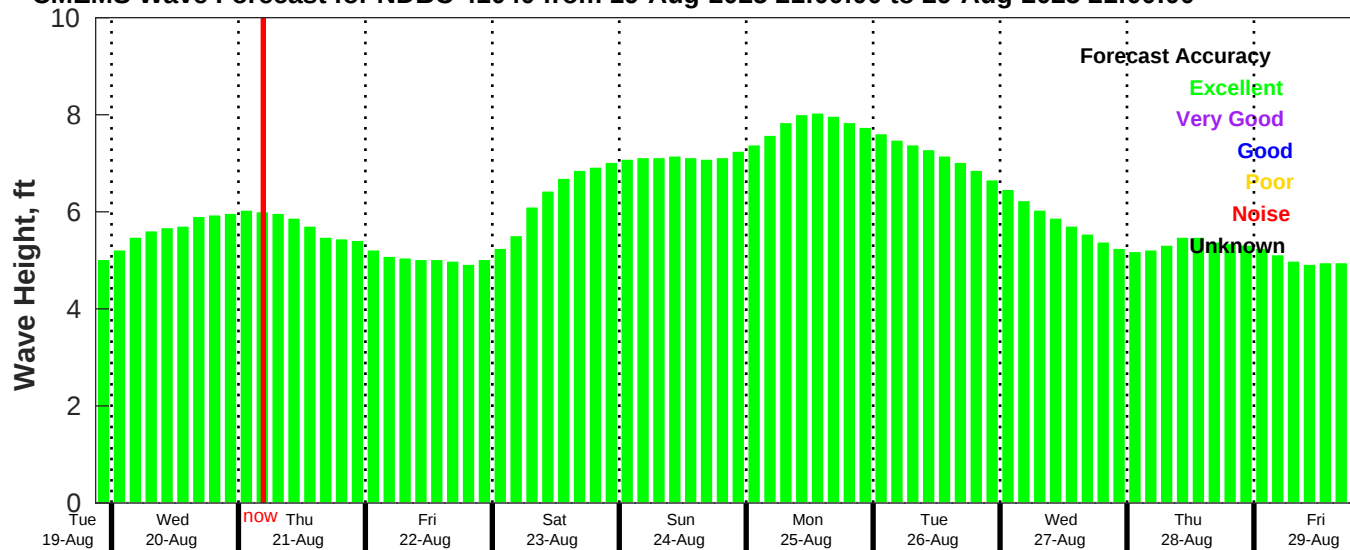
CMEMS Wave Forecast for NDBC 41040 from 19-Aug-2025 21:00:00 to 29-Aug-2025 21:00:00
