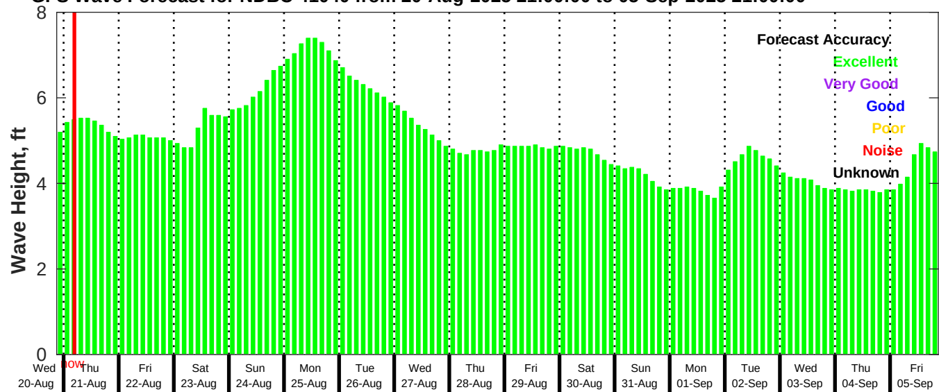
GFS Wave Forecast for NDBC 41040 from 20-Aug-2025 21:00:00 to 05-Sep-2025 21:00:00
