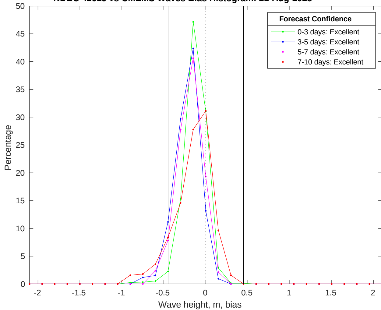
NDBC 42019 vs CMEMS Waves Bias Histogram: 21-Aug-2025
