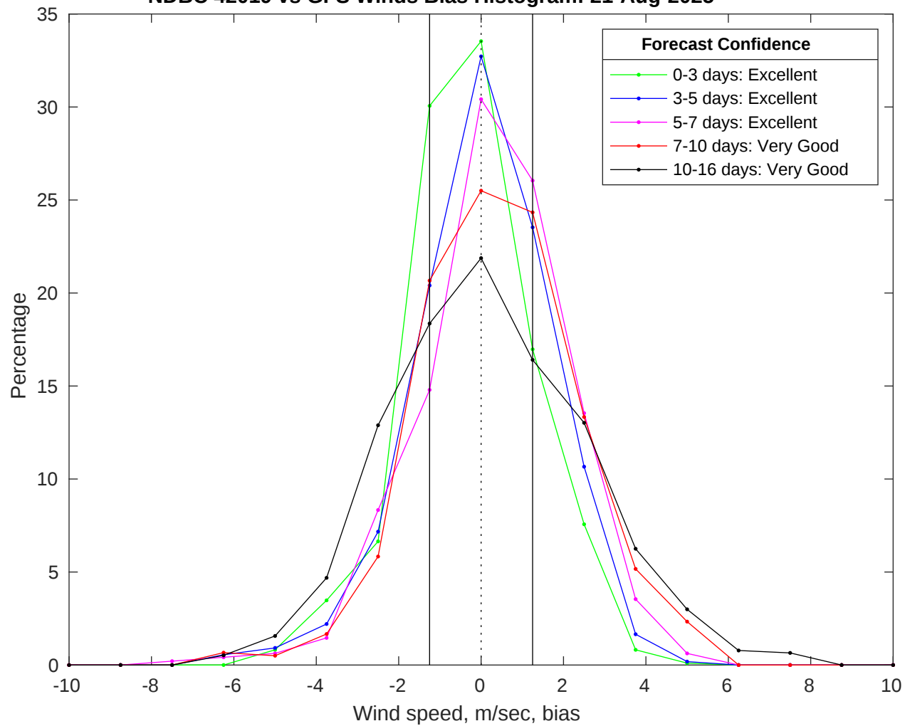
NDBC 42019 vs GFS Winds Bias Histogram: 21-Aug-2025
