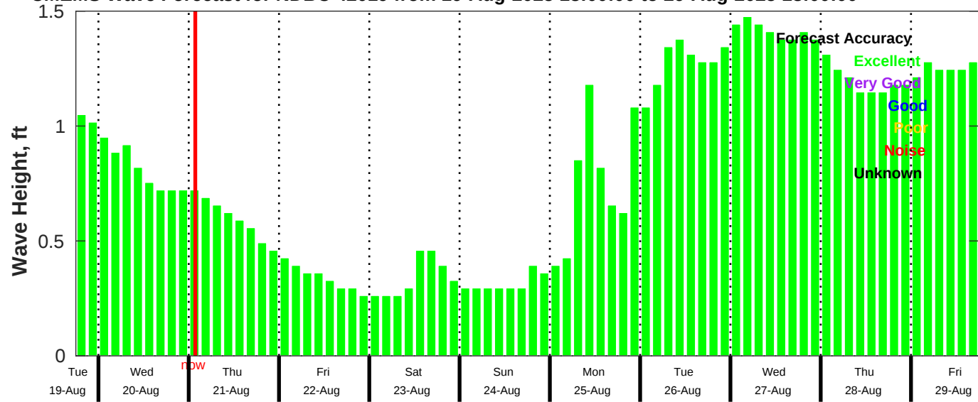
CMEMS Wave Forecast for NDBC 42019 from 19-Aug-2025 18:00:00 to 29-Aug-2025 18:00:00
