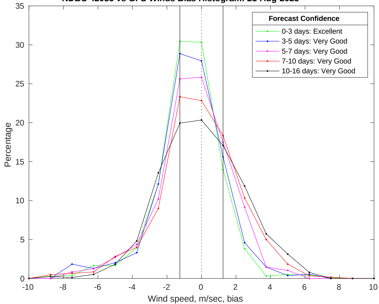
NDBC 42035 vs GFS Winds Bias Histogram: 21-Aug-2025
