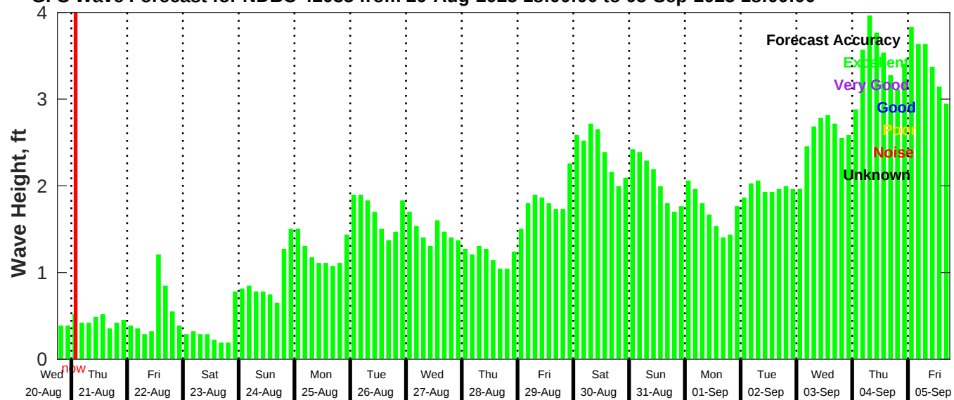
GFS Wave Forecast for NDBC 42035 from 20-Aug-2025 18:00:00 to 05-Sep-2025 18:00:00
