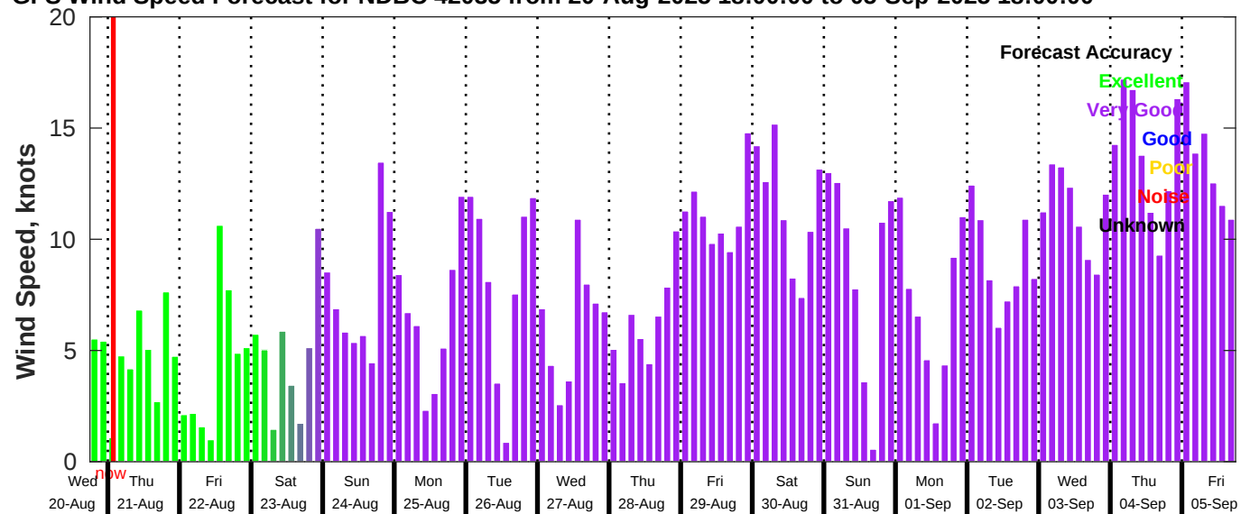
GFS Wind Speed Forecast for NDBC 42035 from 20-Aug-2025 18:00:00 to 05-Sep-2025 18:00:00
