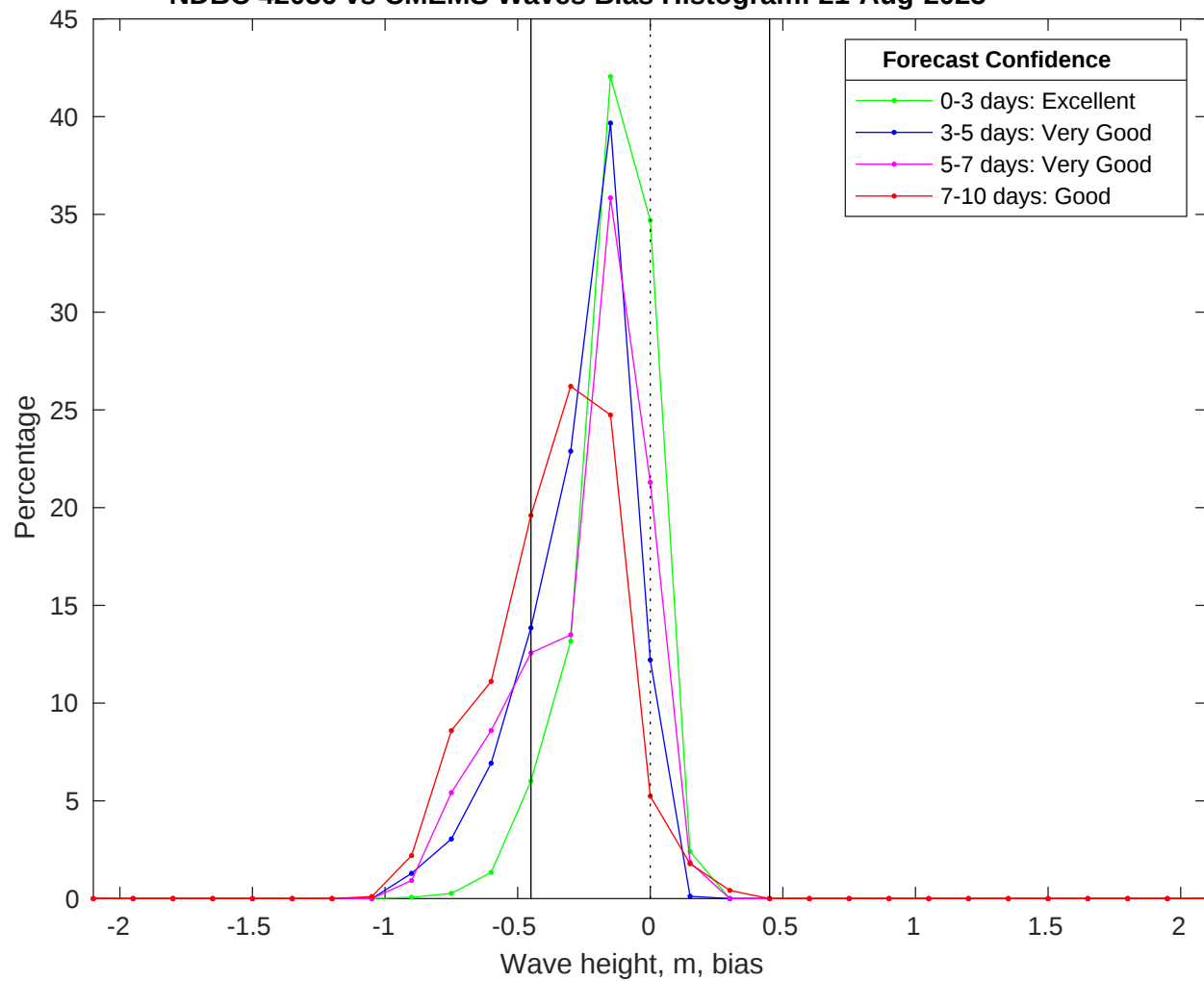
NDBC 42036 vs CMEMS Waves Bias Histogram: 21-Aug-2025
