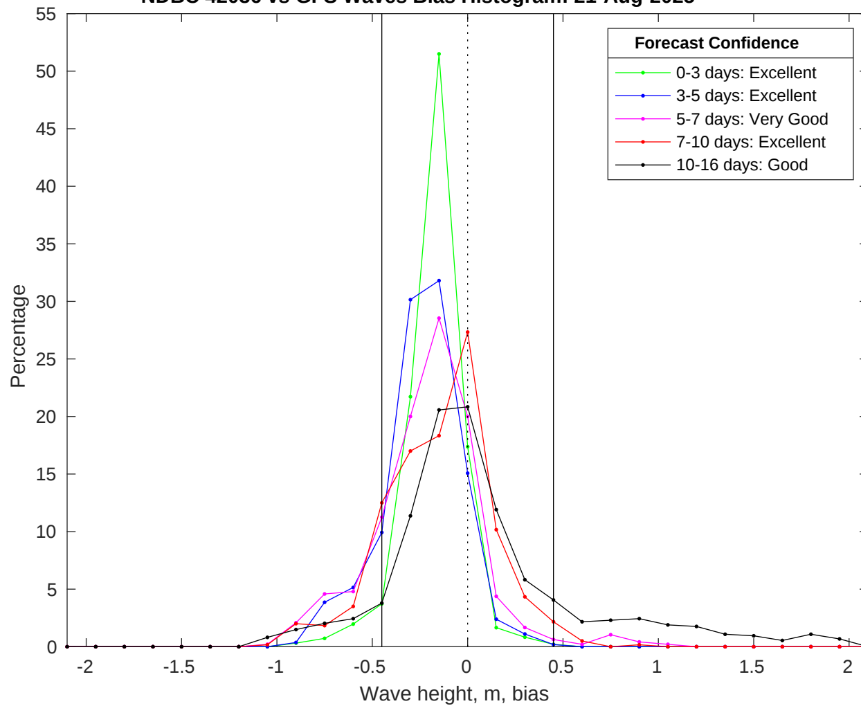
NDBC 42036 vs GFS Waves Bias Histogram: 21-Aug-2025
