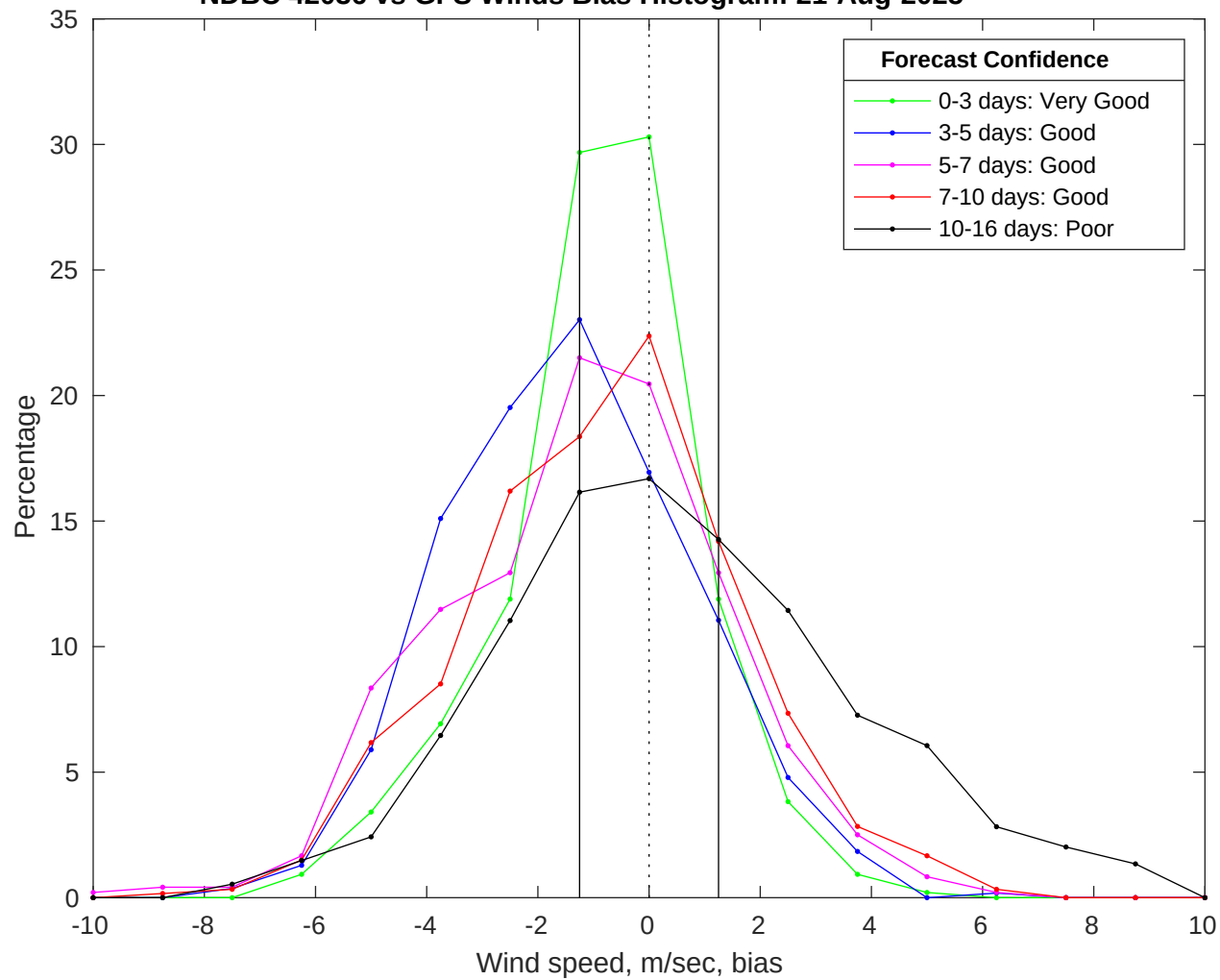
NDBC 42036 vs GFS Winds Bias Histogram: 21-Aug-2025
