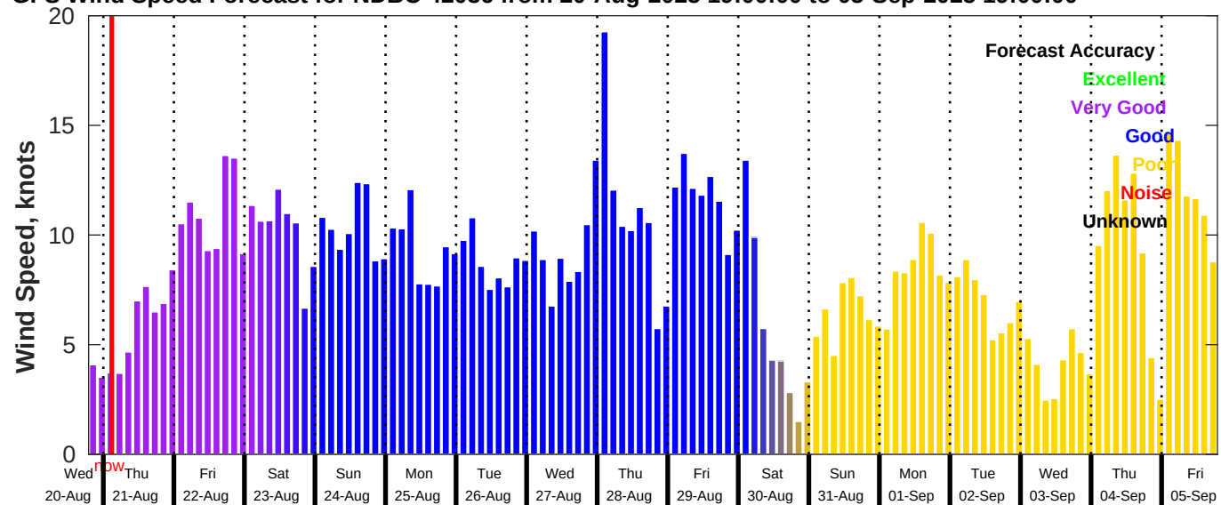
GFS Wind Speed Forecast for NDBC 42036 from 20-Aug-2025 19:00:00 to 05-Sep-2025 19:00:00
