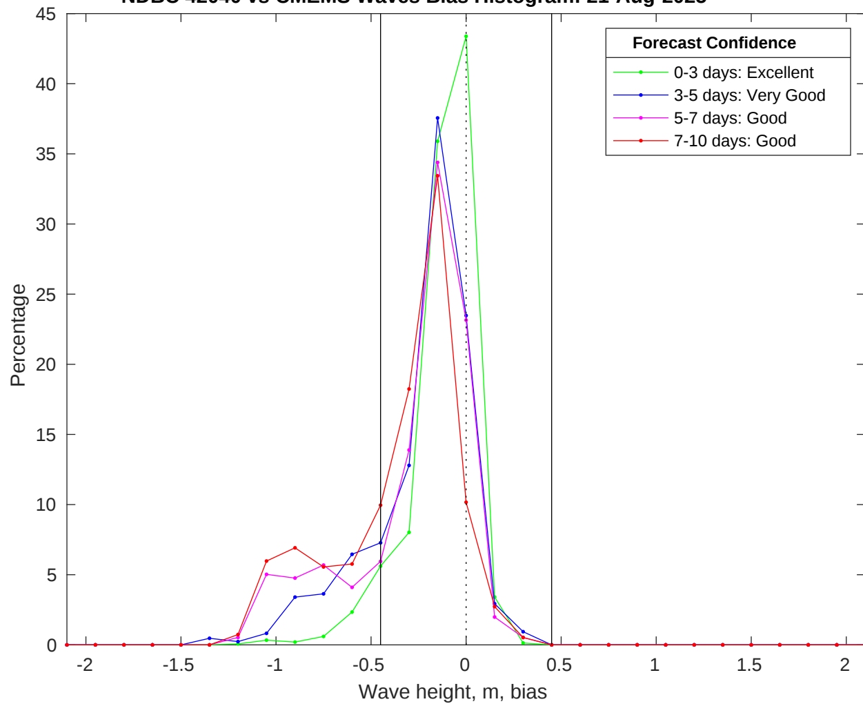
NDBC 42040 vs CMEMS Waves Bias Histogram: 21-Aug-2025
