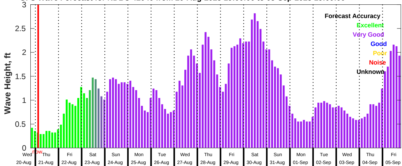
GFS Wave Forecast for NDBC 42040 from 20-Aug-2025 19:00:00 to 05-Sep-2025 19:00:00
