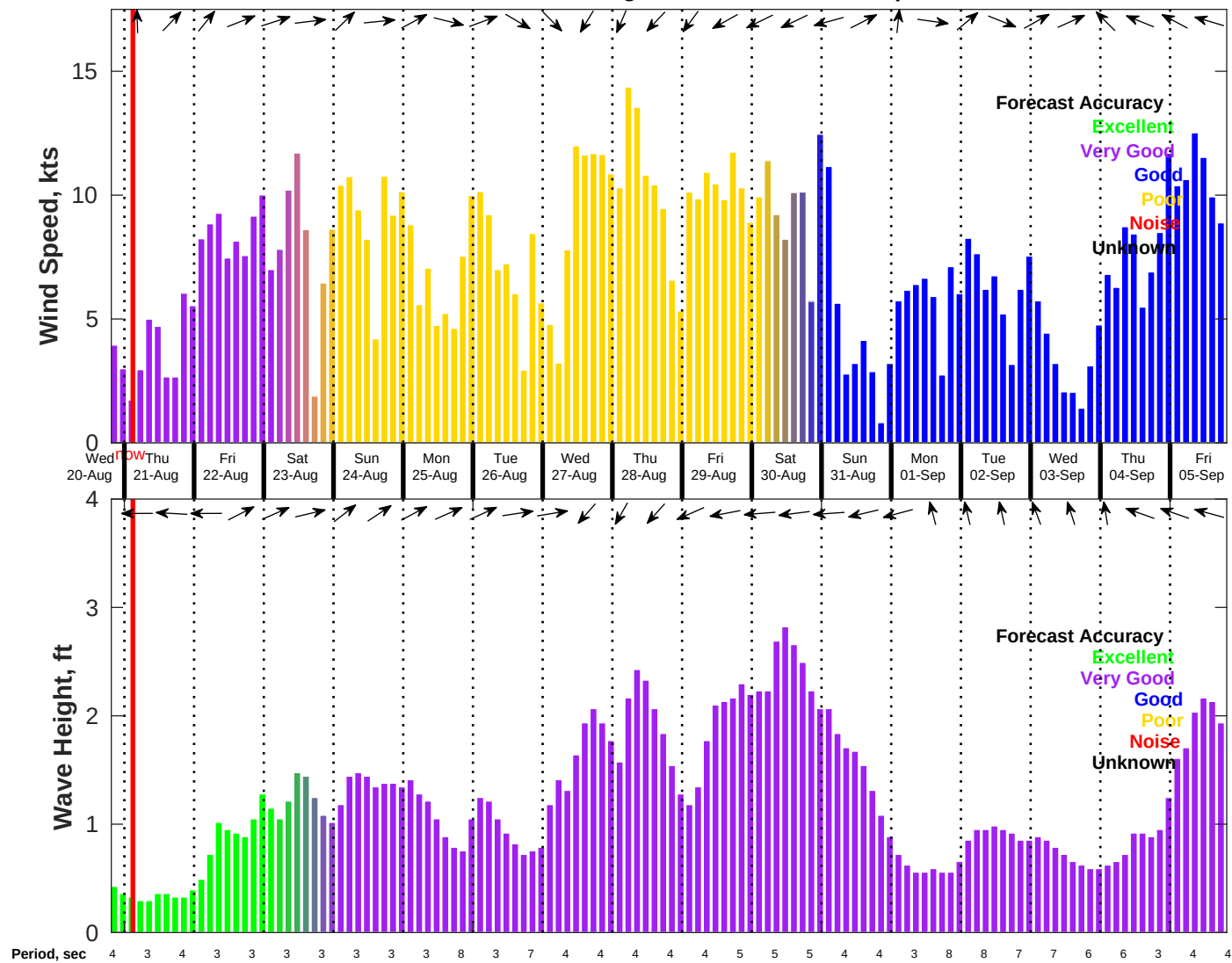
Wind & Wave Forecast for NDBC 42040 from 20-Aug-2025 19:00:00 to 05-Sep-2025 19:00:00
