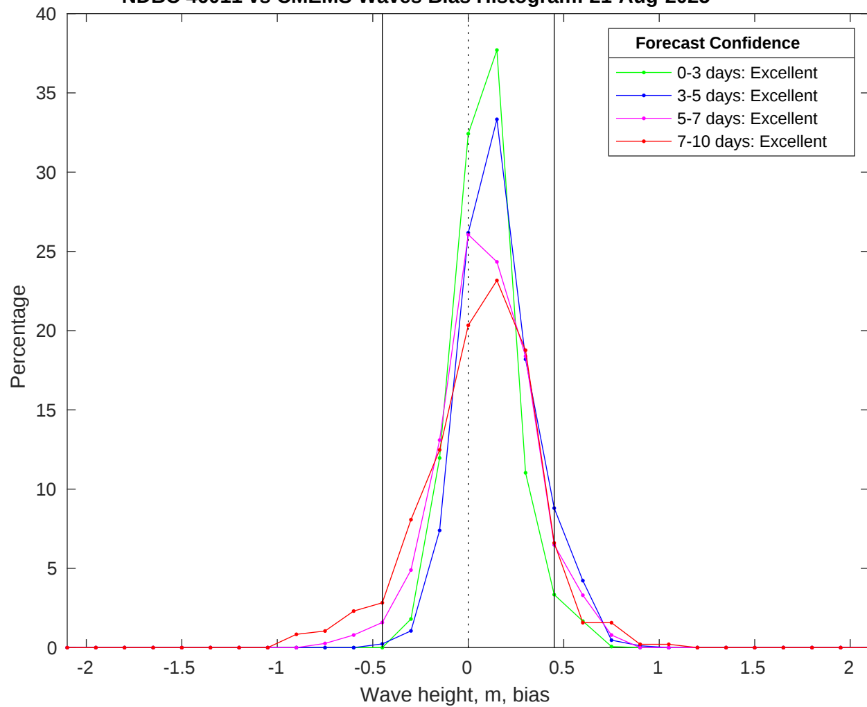
NDBC 46011 vs CMEMS Waves Bias Histogram: 21-Aug-2025
