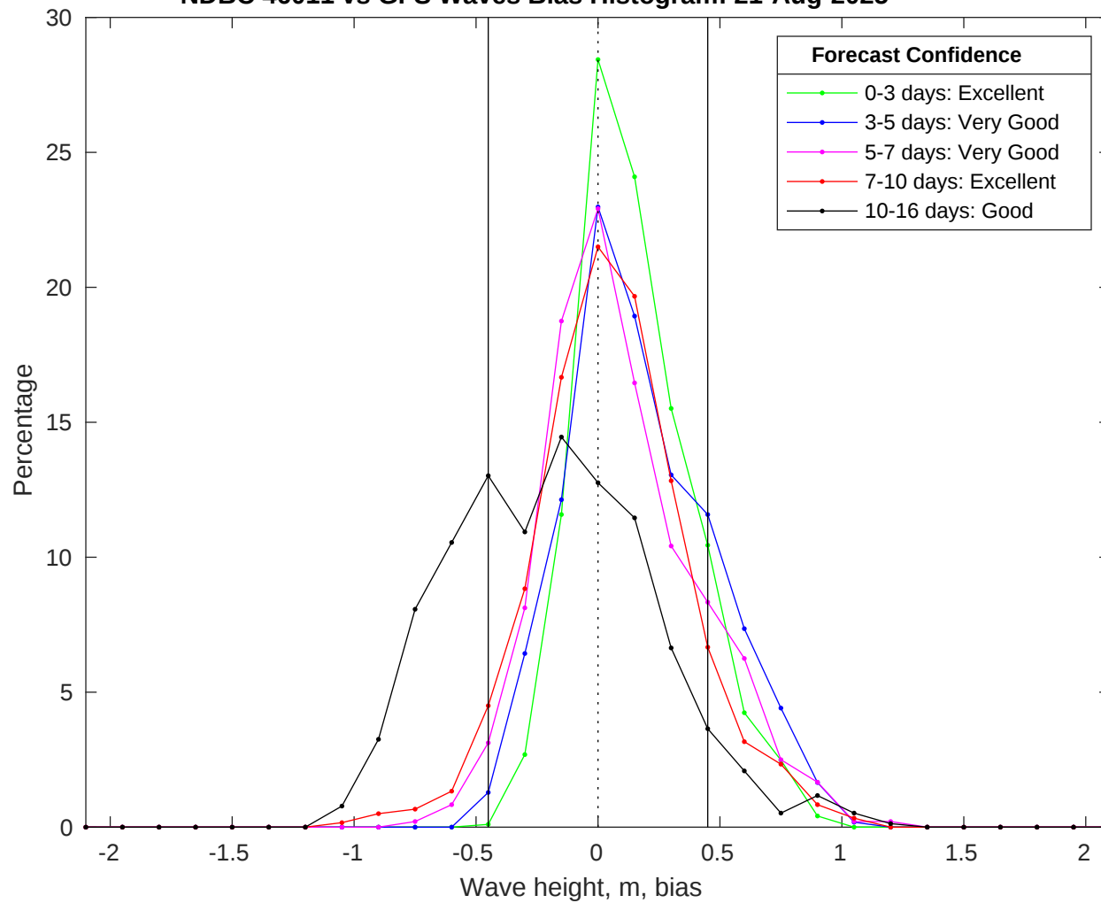
NDBC 46011 vs GFS Waves Bias Histogram: 21-Aug-2025
