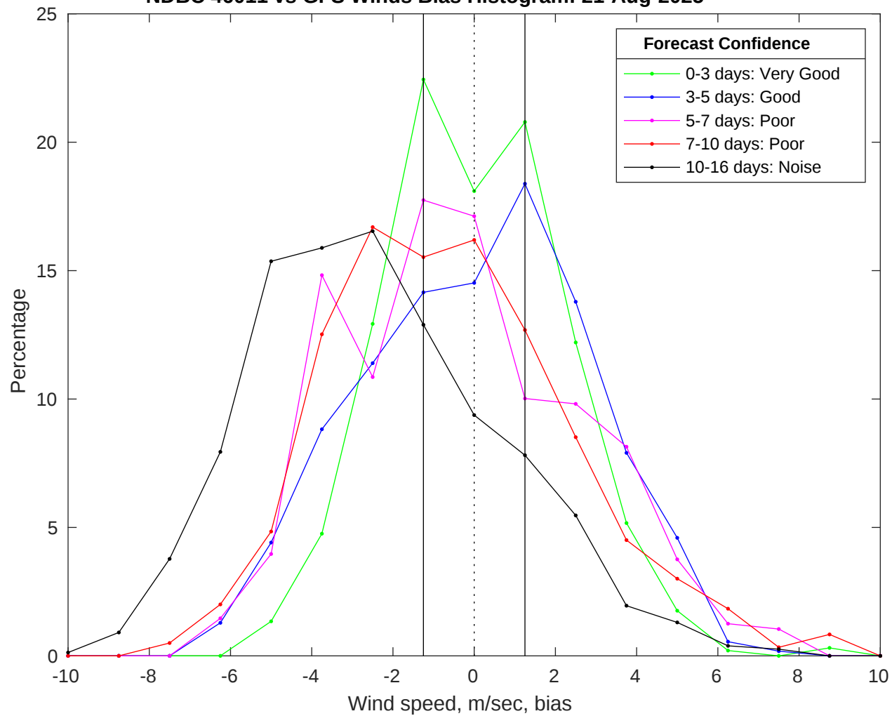
NDBC 46011 vs GFS Winds Bias Histogram: 21-Aug-2025
