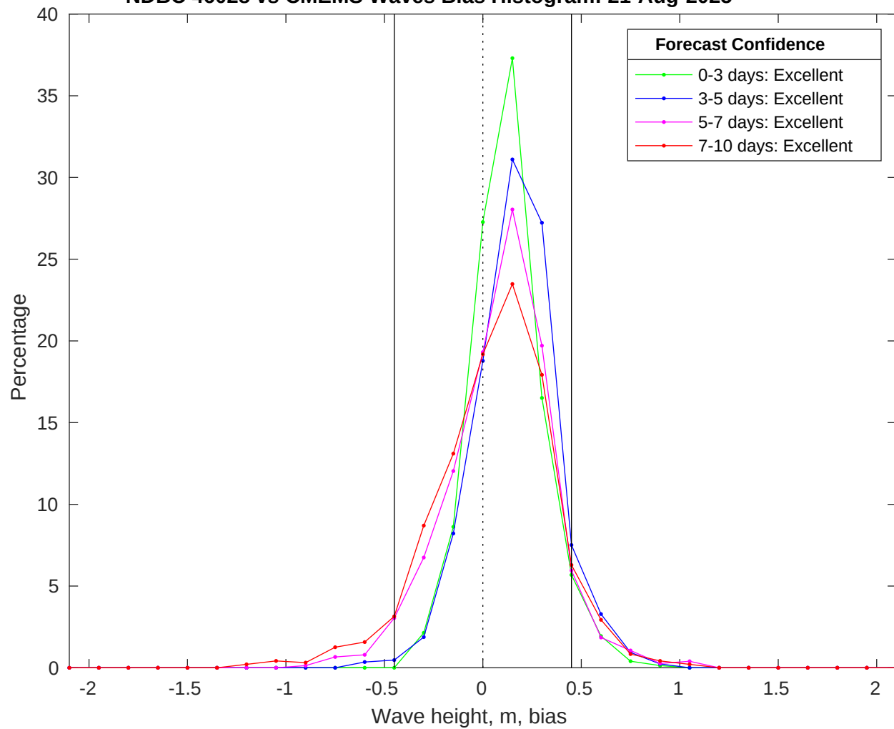
NDBC 46028 vs CMEMS Waves Bias Histogram: 21-Aug-2025
