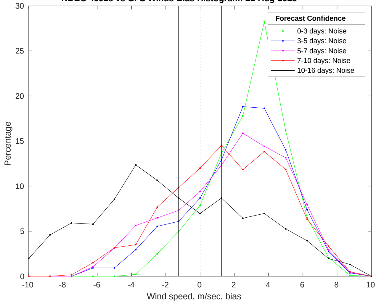
NDBC 46028 vs GFS Winds Bias Histogram: 21-Aug-2025
