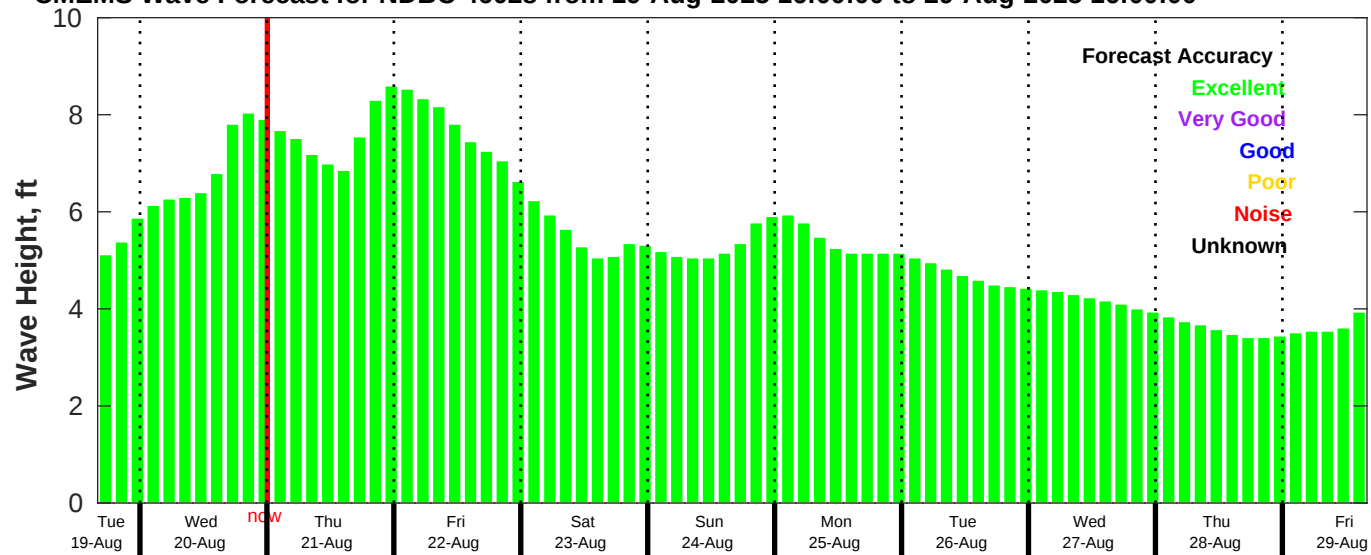
CMEMS Wave Forecast for NDBC 46028 from 19-Aug-2025 16:00:00 to 29-Aug-2025 16:00:00
