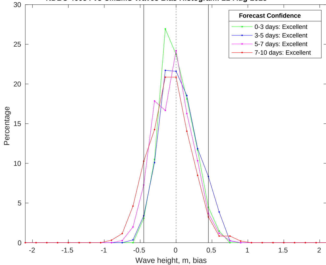
NDBC 46054 vs CMEMS Waves Bias Histogram: 21-Aug-2025
