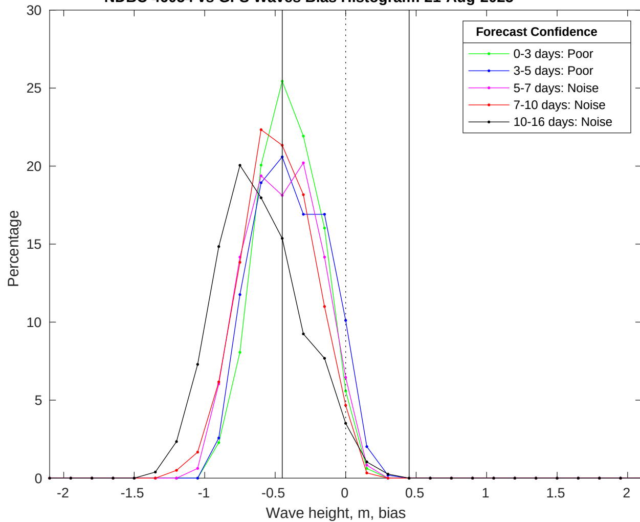
NDBC 46054 vs GFS Waves Bias Histogram: 21-Aug-2025
